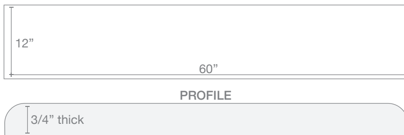
12" Bench Top - 12" wide x 60" long, 2 long finished edges, 1 short finished edge if requested.
